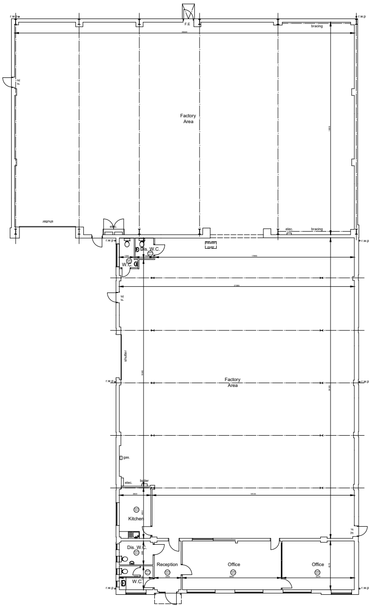
Ground Floor Plan - GIA: 1217.6 sq m. (13106 sq ft.)
